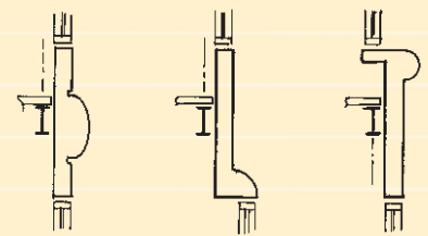
Fig. B-5—A bullnose with reveals at top and bottom. Fig. B-6—A half bullnose. Fig. B-7—A bullnose featuring a return.
