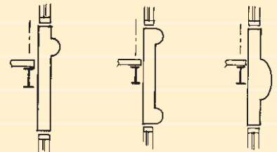
Fig. B-2—A typical bullnose. Fig. B-3—A double bullnose. Fig. B-4—An elliptical bullnose.
